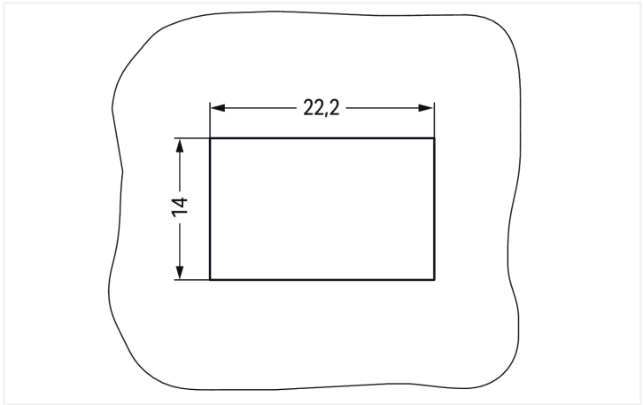
Méretetek mm-ben Plate thickness: 0.5 ... 2 mm Cutout tolerance: + 0.1 mm
