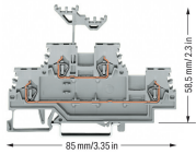
Double-deck marker carrier (height including marker carrier)
