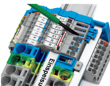
Tool-operated N-disconnect slide link
